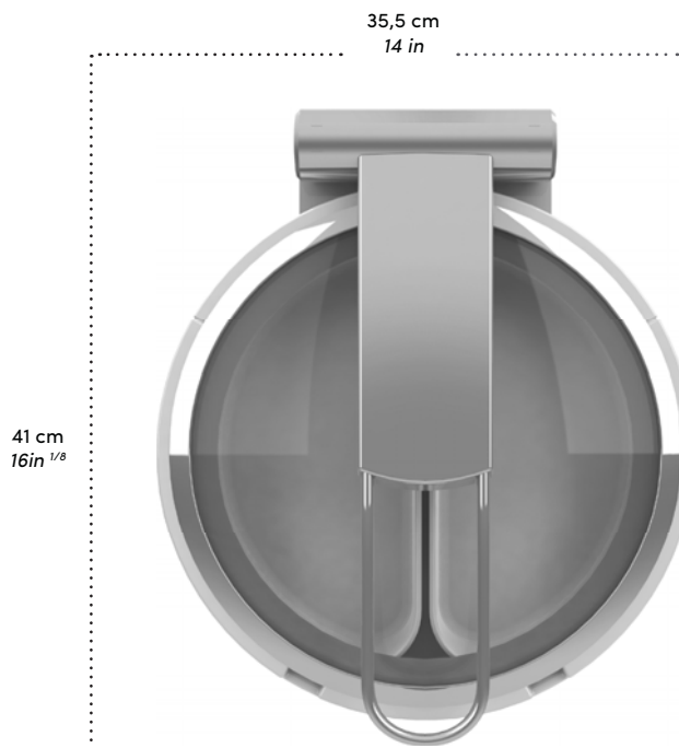
Ø 35,5 cm - P 41 cm - H 15 cm Ø 14 in - D 16 in 1/8 - H 5 in 7/8
